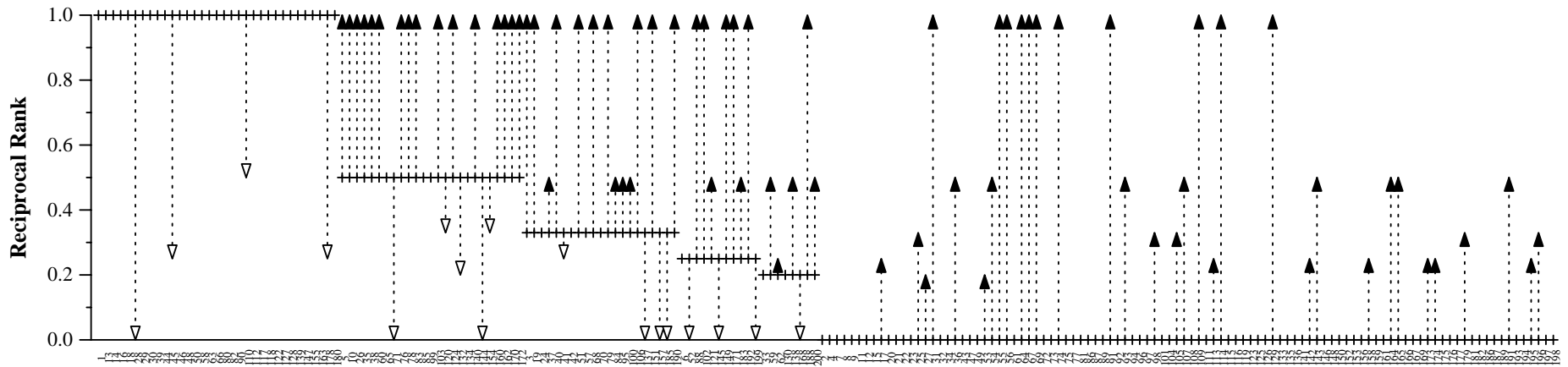
Question number by descending median Run scores vs. median scores by question for run mds08q1
