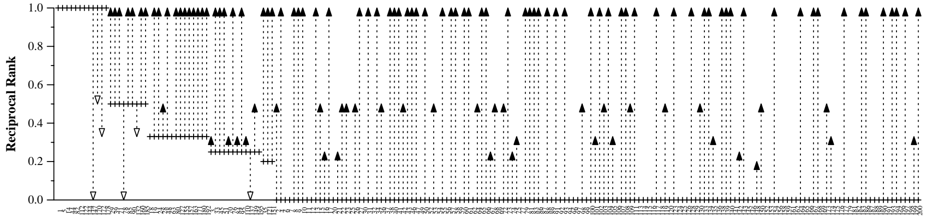
Question number by descending median Run scores vs. median scores by question for run SMUNLP1
