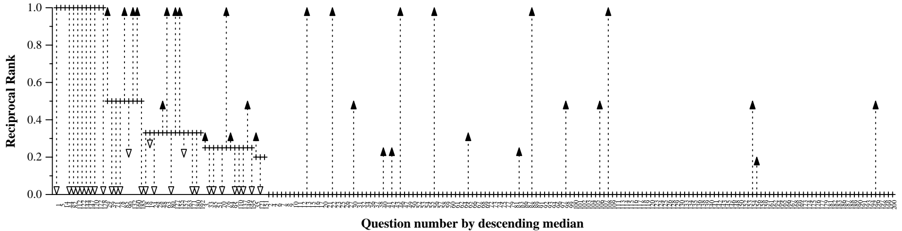
Run scores vs. median scores by question for run INQ638
