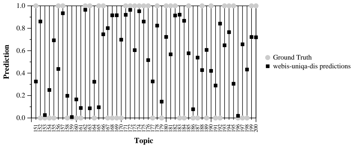
Per-topic webis-uniqa-dis Prediction and Ground Truth
