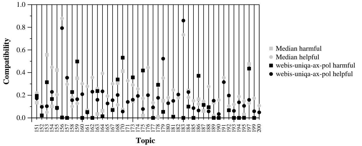
Per-topic Compatibility with Harmful and Helpful for webis-uniqa-ax-pol and Median
