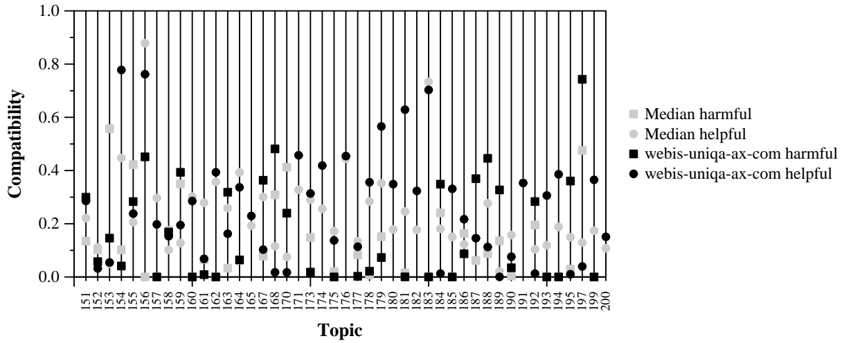
Per-topic Compatibility with Harmful and Helpful for webis-uniqa-ax-com and Median
