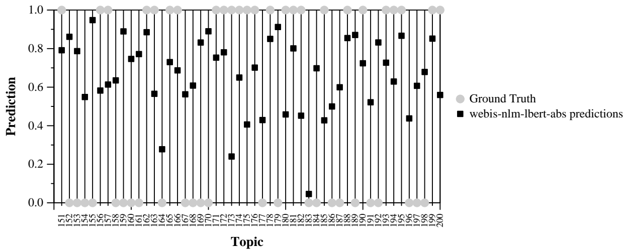
Per-topic webis-nlm-lbert-abs Prediction and Ground Truth
