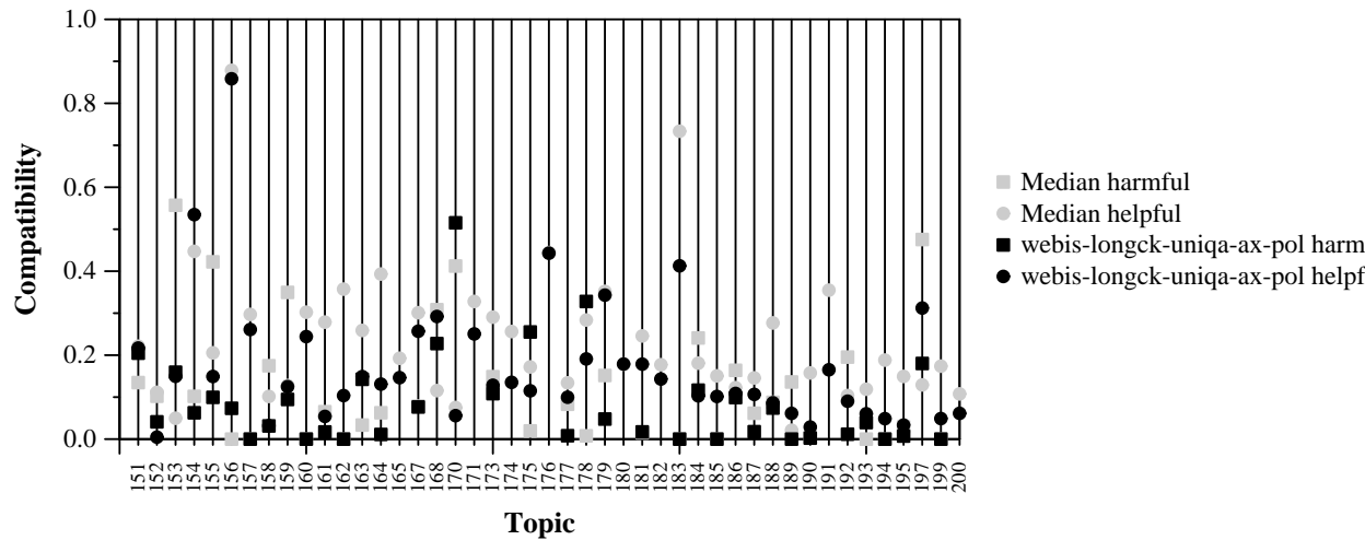
Per-topic Compatibility with Harmful and Helpful for webis-longck-uniqa-ax-pol and Median
