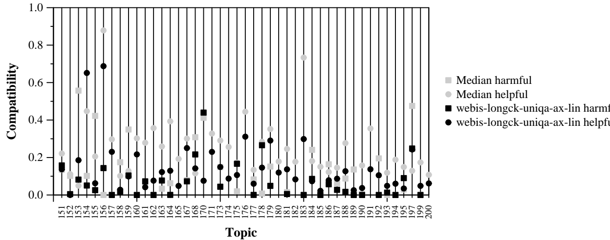
Per-topic Compatibility with Harmful and Helpful for webis-longck-uniqa-ax-lin and Median
