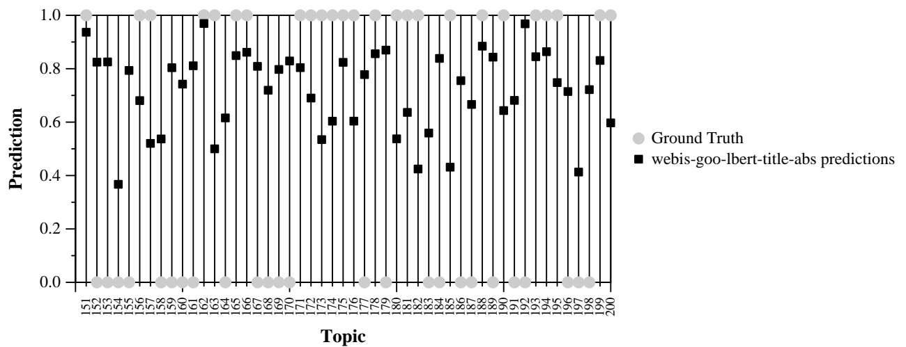
Per-topic webis-goo-lbert-title-abs Prediction and Ground Truth
