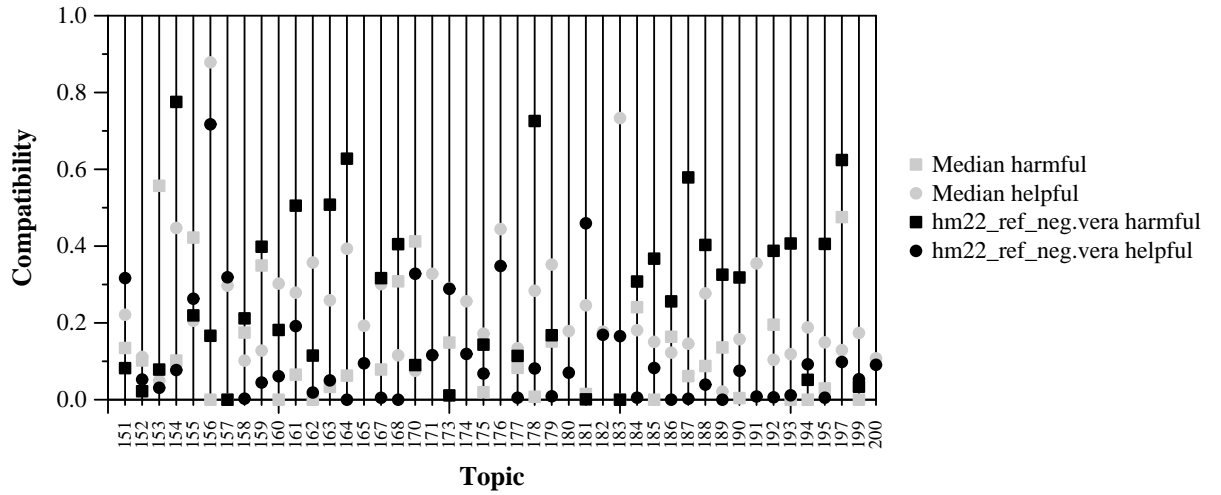
Per-topic Compatibility with Harmful and Helpful for hm22_ref_neg.vera and Median
