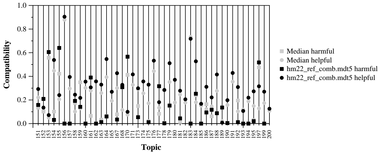
Per-topic Compatibility with Harmful and Helpful for hm22_ref_comb.mdt5 and Median
