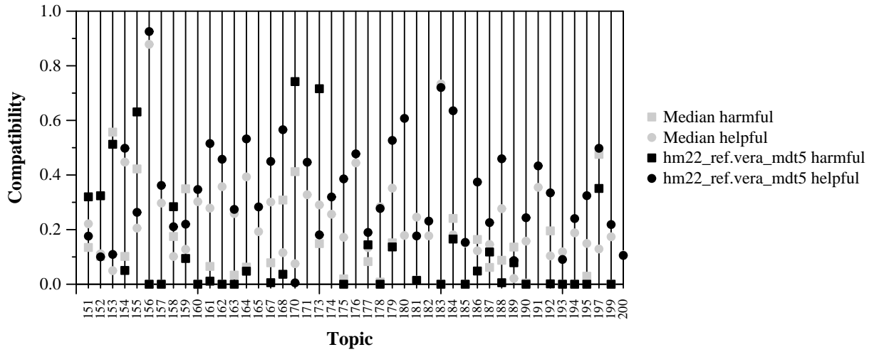
Per-topic Compatibility with Harmful and Helpful for hm22_ref.vera_mdt5 and Median
