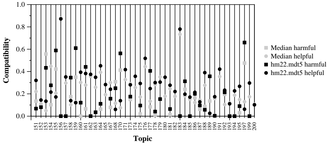
Per-topic Compatibility with Harmful and Helpful for hm22.mdt5 and Median
