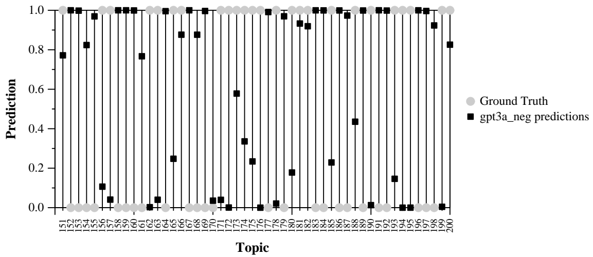
Per-topic gpt3a_neg Prediction and Ground Truth
