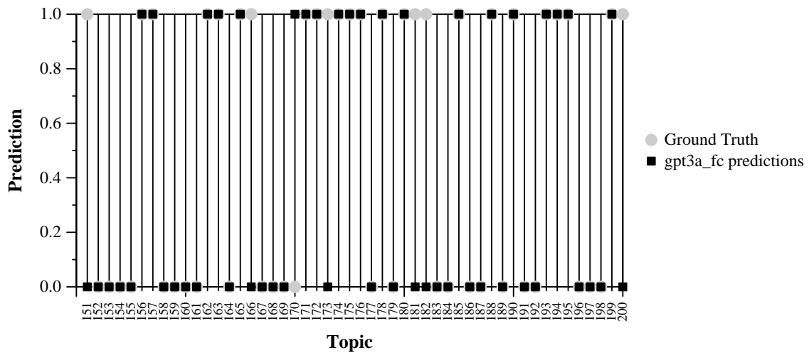
Per-topic gpt3a_fc Prediction and Ground Truth
