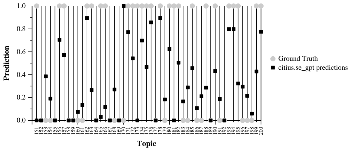
Per-topic citius.se_gpt Prediction and Ground Truth
