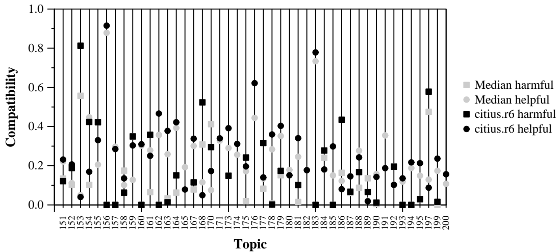
Per-topic Compatibility with Harmful and Helpful for citius.r6 and Median
