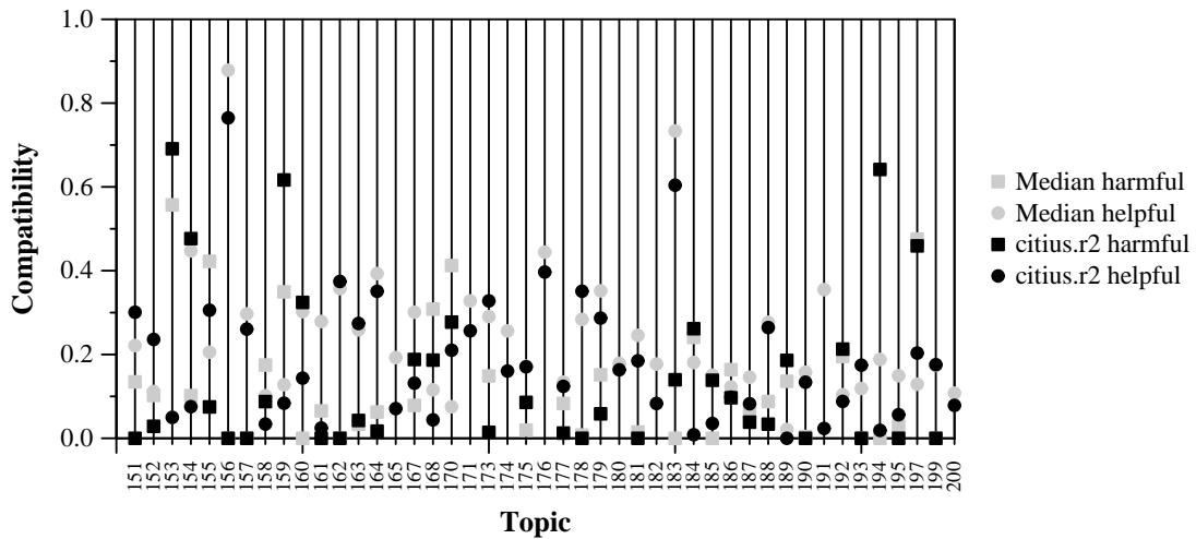
Per-topic Compatibility with Harmful and Helpful for citius.r2 and Median
