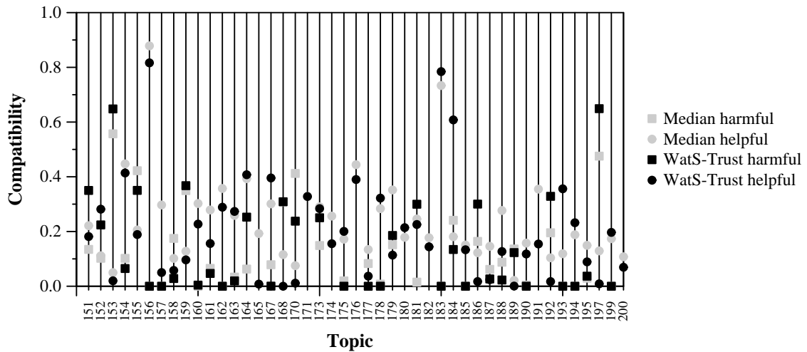
Per-topic Compatibility with Harmful and Helpful for WatS-Trust and Median
