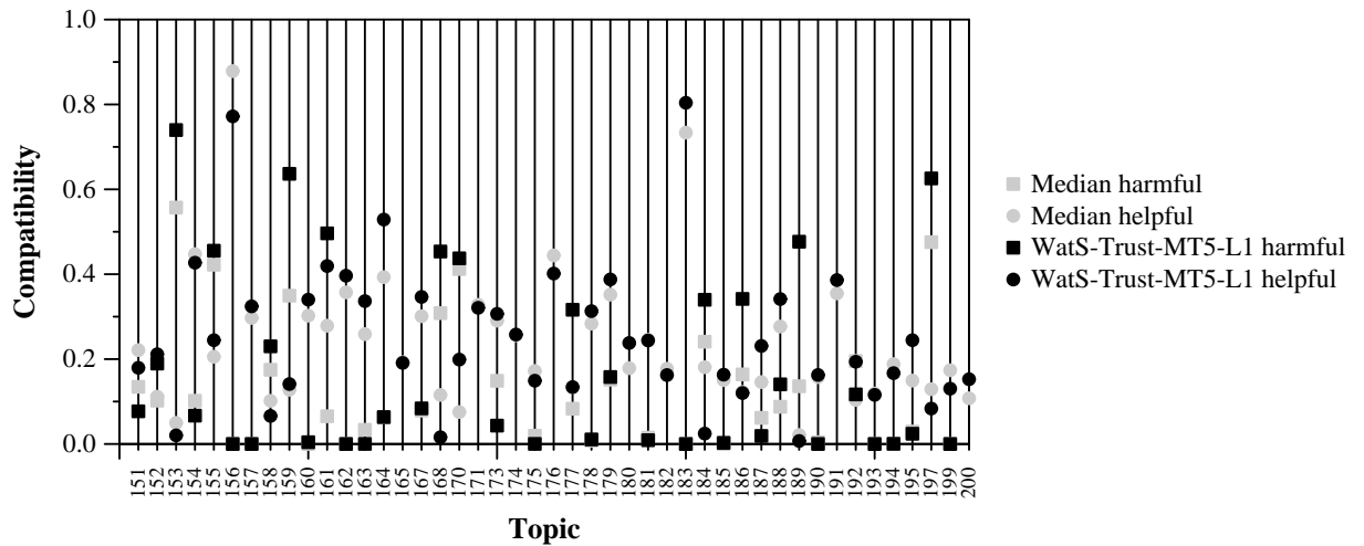
Per-topic Compatibility with Harmful and Helpful for WatS-Trust-MT5-L1 and Median
