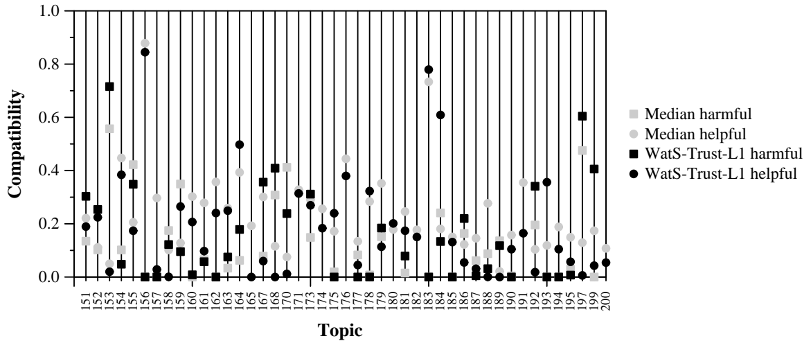
Per-topic Compatibility with Harmful and Helpful for WatS-Trust-L1 and Median
