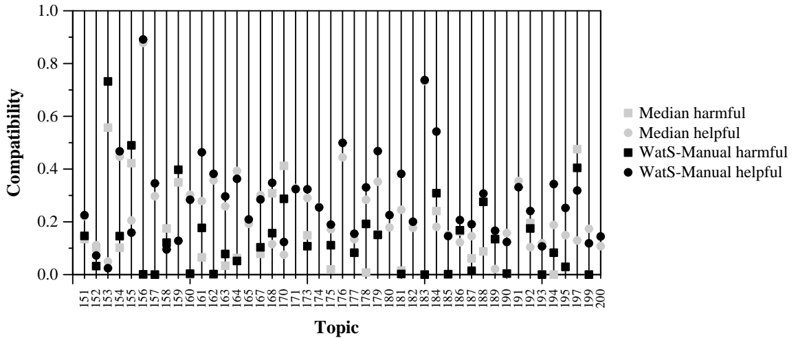
Per-topic Compatibility with Harmful and Helpful for WatS-Manual and Median
