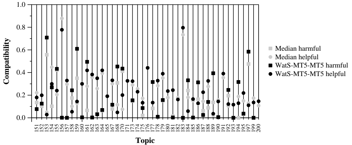
Per-topic Compatibility with Harmful and Helpful for WatS-MT5-MT5 and Median
