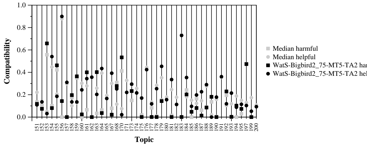
Per-topic Compatibility with Harmful and Helpful for WatS-Bigbird2_75-MT5-TA2 and Median
