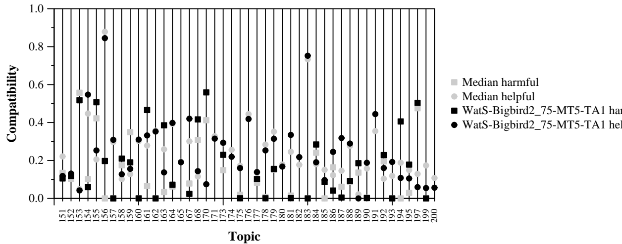
Per-topic Compatibility with Harmful and Helpful for WatS-Bigbird2_75-MT5-TA1 and Median
