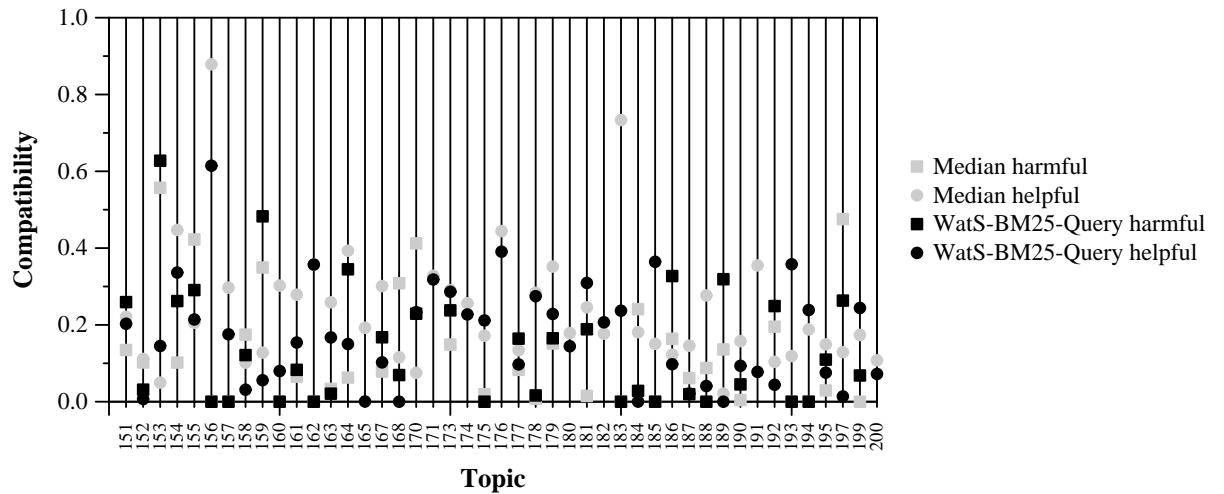
Per-topic Compatibility with Harmful and Helpful for WatS-BM25-Query and Median
