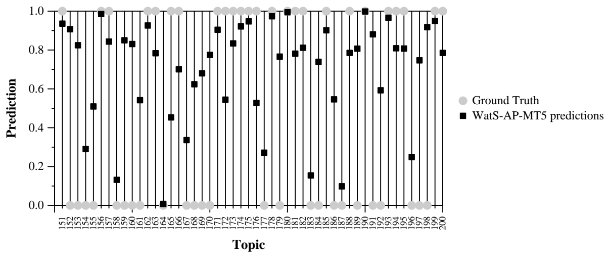
Per-topic WatS-AP-MT5 Prediction and Ground Truth
