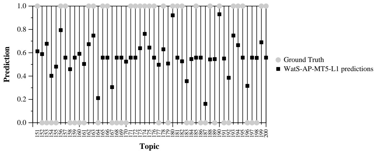
Per-topic WatS-AP-MT5-L1 Prediction and Ground Truth
