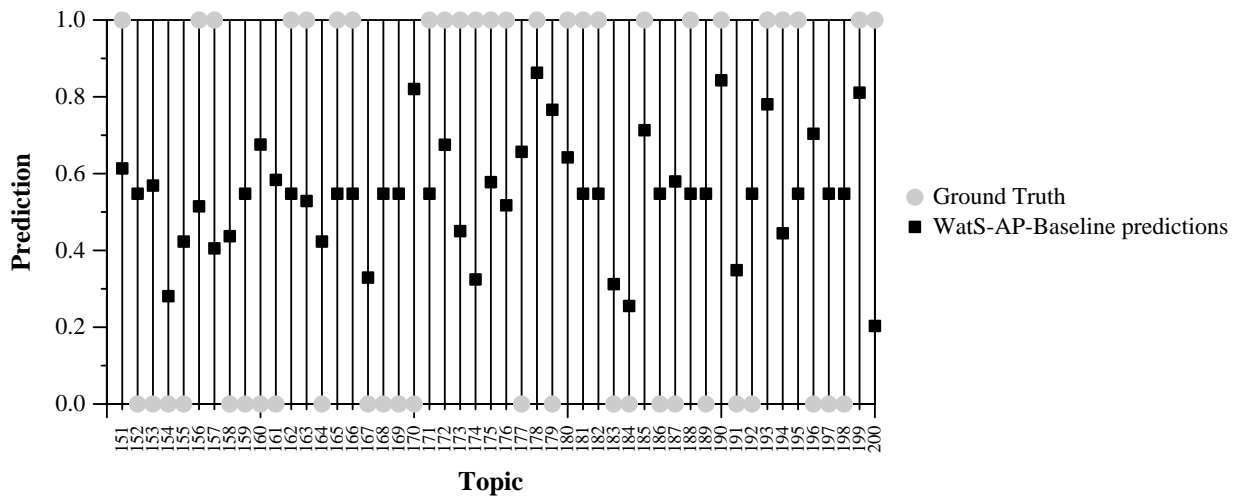
Per-topic WatS-AP-Baseline Prediction and Ground Truth
