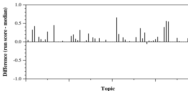
Per-topic difference from median NDCG@10 for Manual runs
