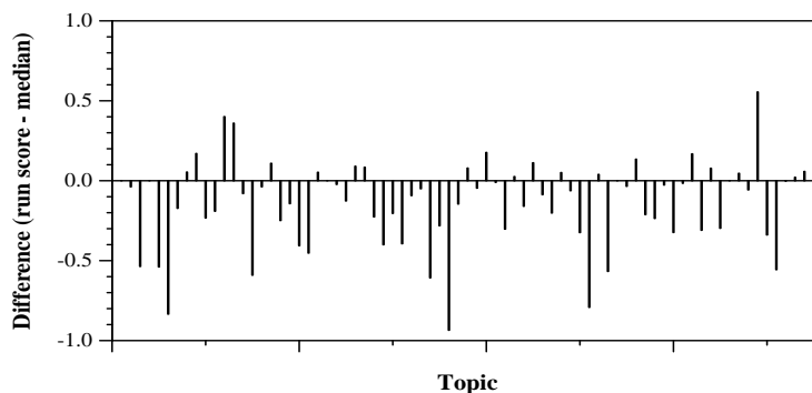
Per-topic difference from median NDCG@10 for Manual runs
