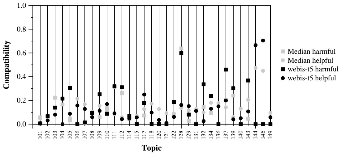
Per-topic Compatibility with Harmful and Helpful for webis-t5 and Median
