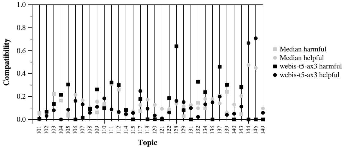
Per-topic Compatibility with Harmful and Helpful for webis-t5-ax3 and Median
