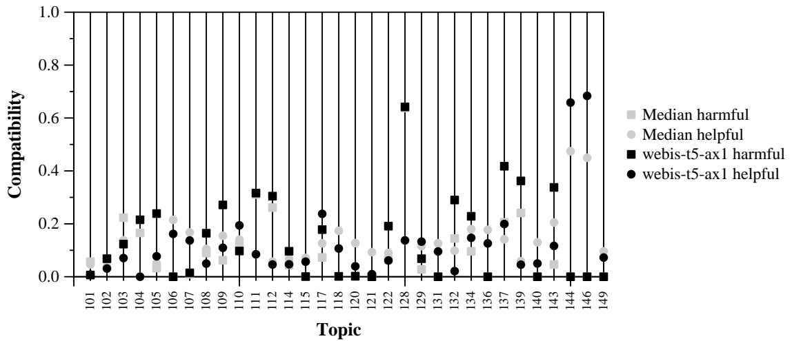
Per-topic Compatibility with Harmful and Helpful for webis-t5-ax1 and Median
