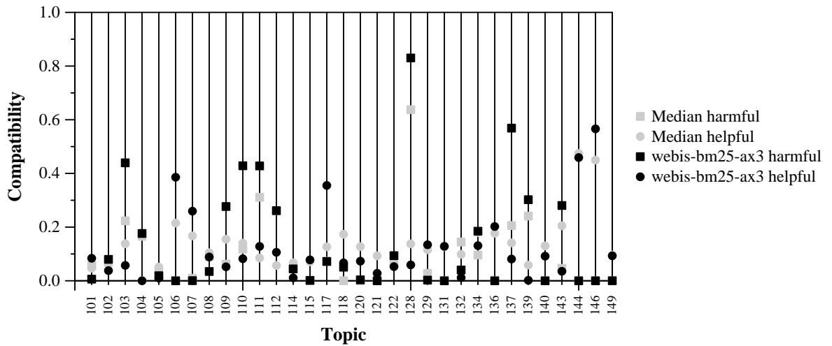
Per-topic Compatibility with Harmful and Helpful for webis-bm25-ax3 and Median
