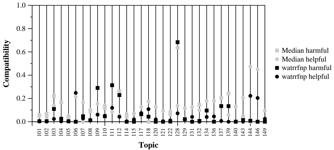
Per-topic Compatibility with Harmful and Helpful for watrrfnp and Median
