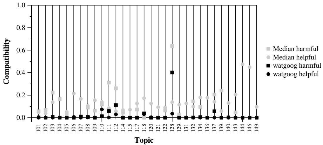
Per-topic Compatibility with Harmful and Helpful for watgoog and Median
