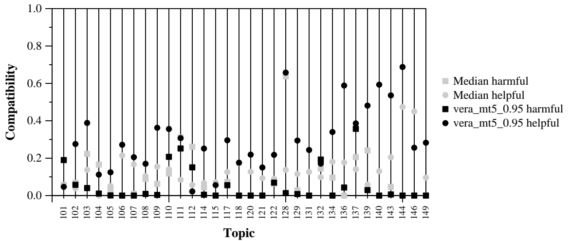
Per-topic Compatibility with Harmful and Helpful for vera_mt5_0.95 and Median
