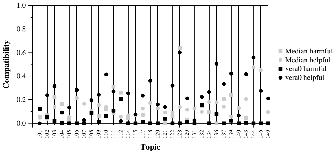
Per-topic Compatibility with Harmful and Helpful for vera0 and Median
