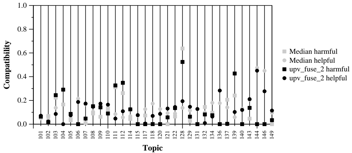
Per-topic Compatibility with Harmful and Helpful for upv_fuse_2 and Median
