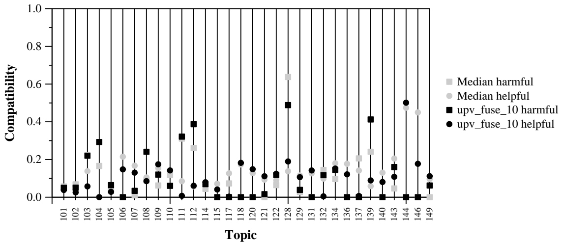
Per-topic Compatibility with Harmful and Helpful for upv_fuse_10 and Median
