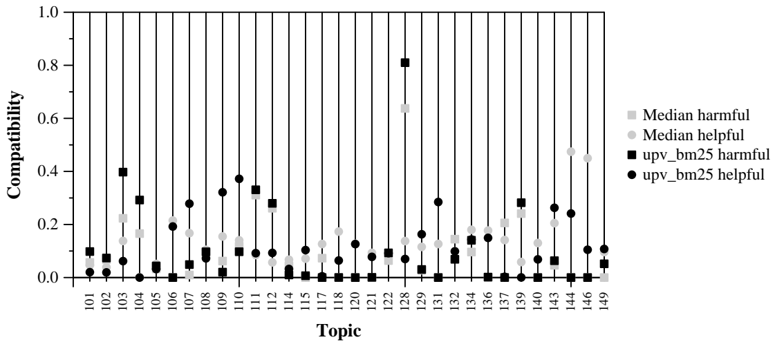
Per-topic Compatibility with Harmful and Helpful for upv_bm25 and Median
