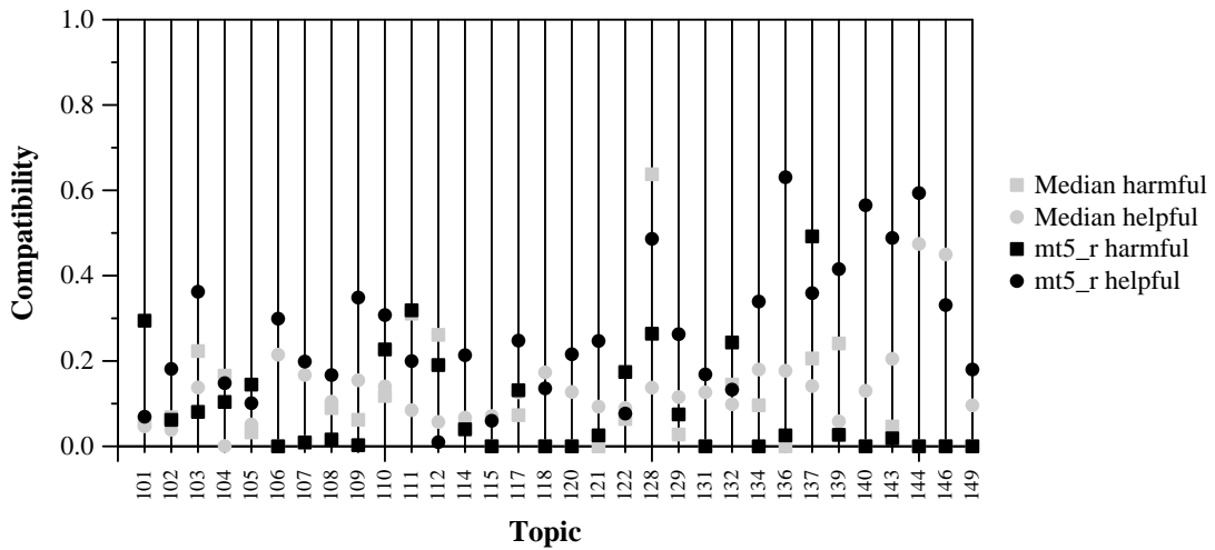
Per-topic Compatibility with Harmful and Helpful for mt5_r and Median
