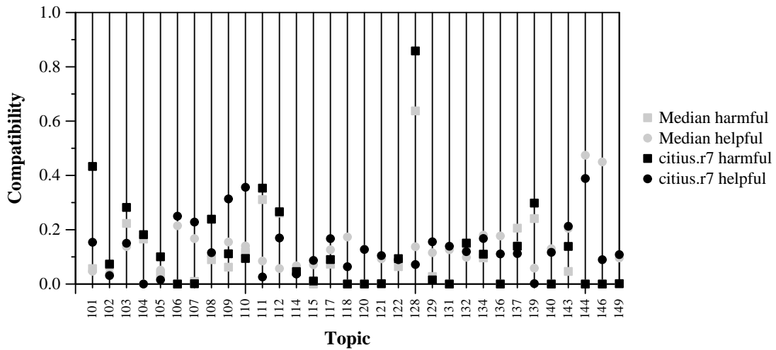
Per-topic Compatibility with Harmful and Helpful for citius.r7 and Median
