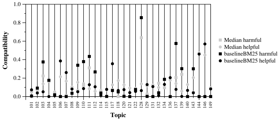
Per-topic Compatibility with Harmful and Helpful for baselineBM25 and Median
