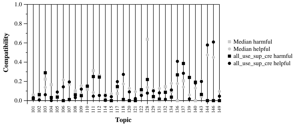
Per-topic Compatibility with Harmful and Helpful for all_use_sup_cre and Median
