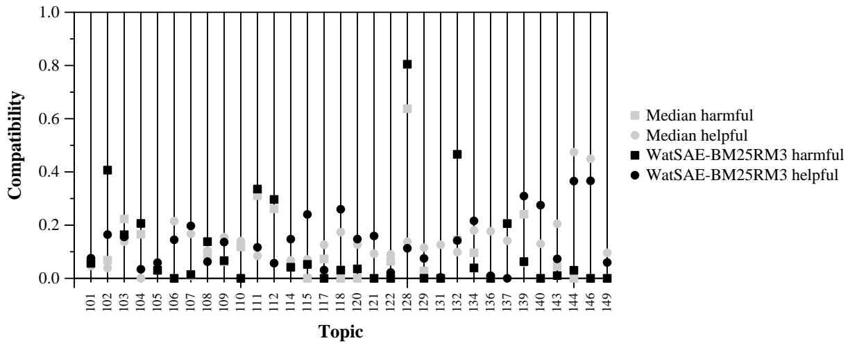
Per-topic Compatibility with Harmful and Helpful for WatSAE-BM25RM3 and Median
