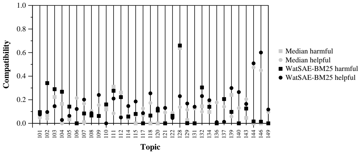
Per-topic Compatibility with Harmful and Helpful for WatSAE-BM25 and Median
