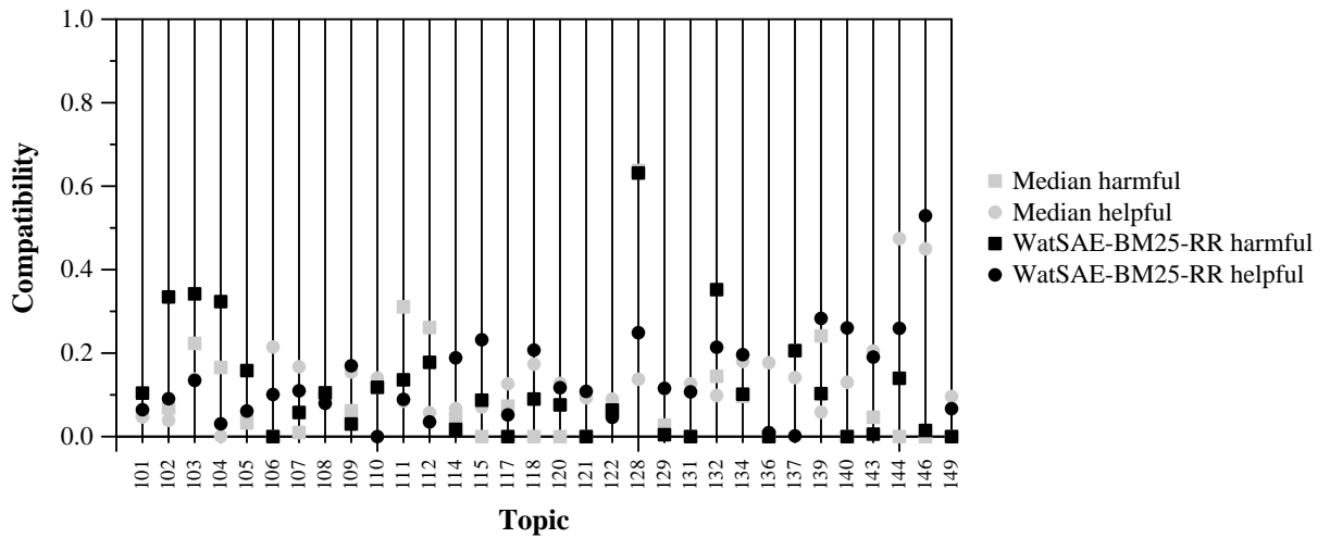
Per-topic Compatibility with Harmful and Helpful for WatSAE-BM25-RR and Median
